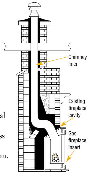
Figure 1. Gas Fireplace Insert in Existing Wood-Burning Fireplace
