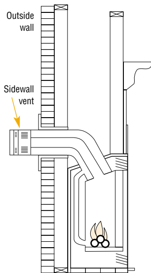
Figure 2. Zero-Clearance Direct-Vent Gas Fireplace
